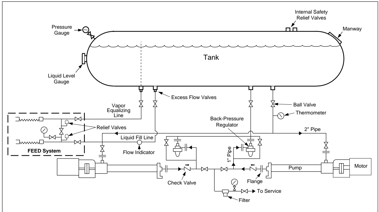
Figure 10. Typical Bulk Storage System
